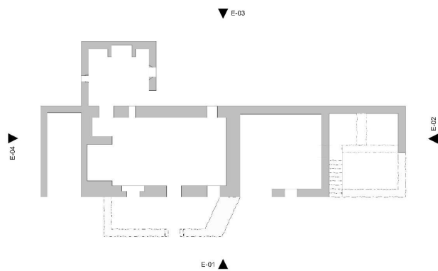
1:100 GF-Ground Floor
