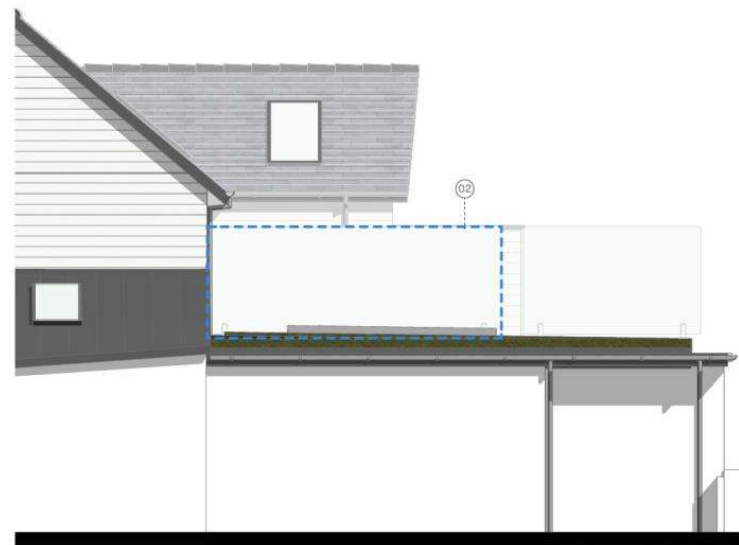
Side Elevation 1:50
