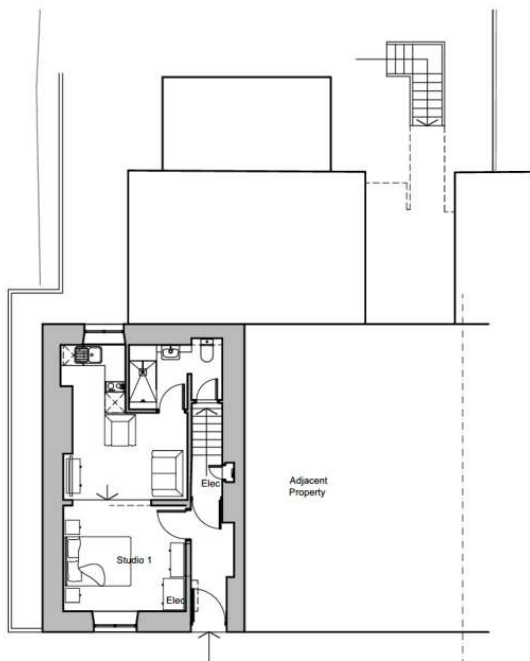
1. Ground Floor Plan
