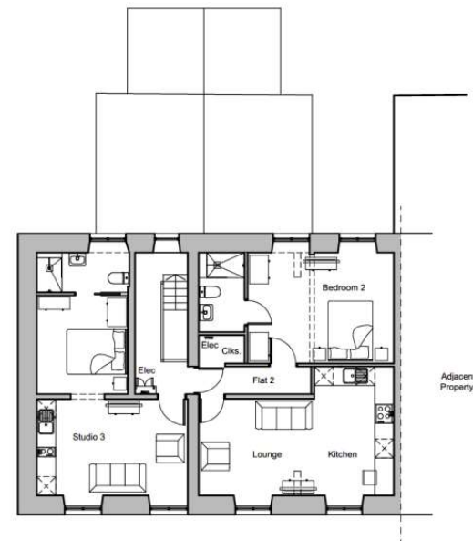
3. Second Floor Plan
